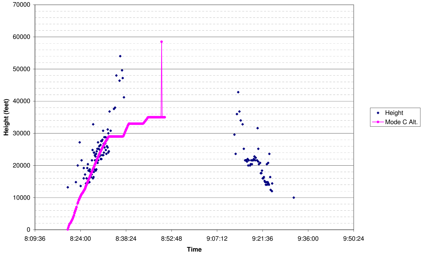
AA77 Pentagon B757 Height & Mode C Altitude, Taken From USAF 84 RADES .XLS Data
