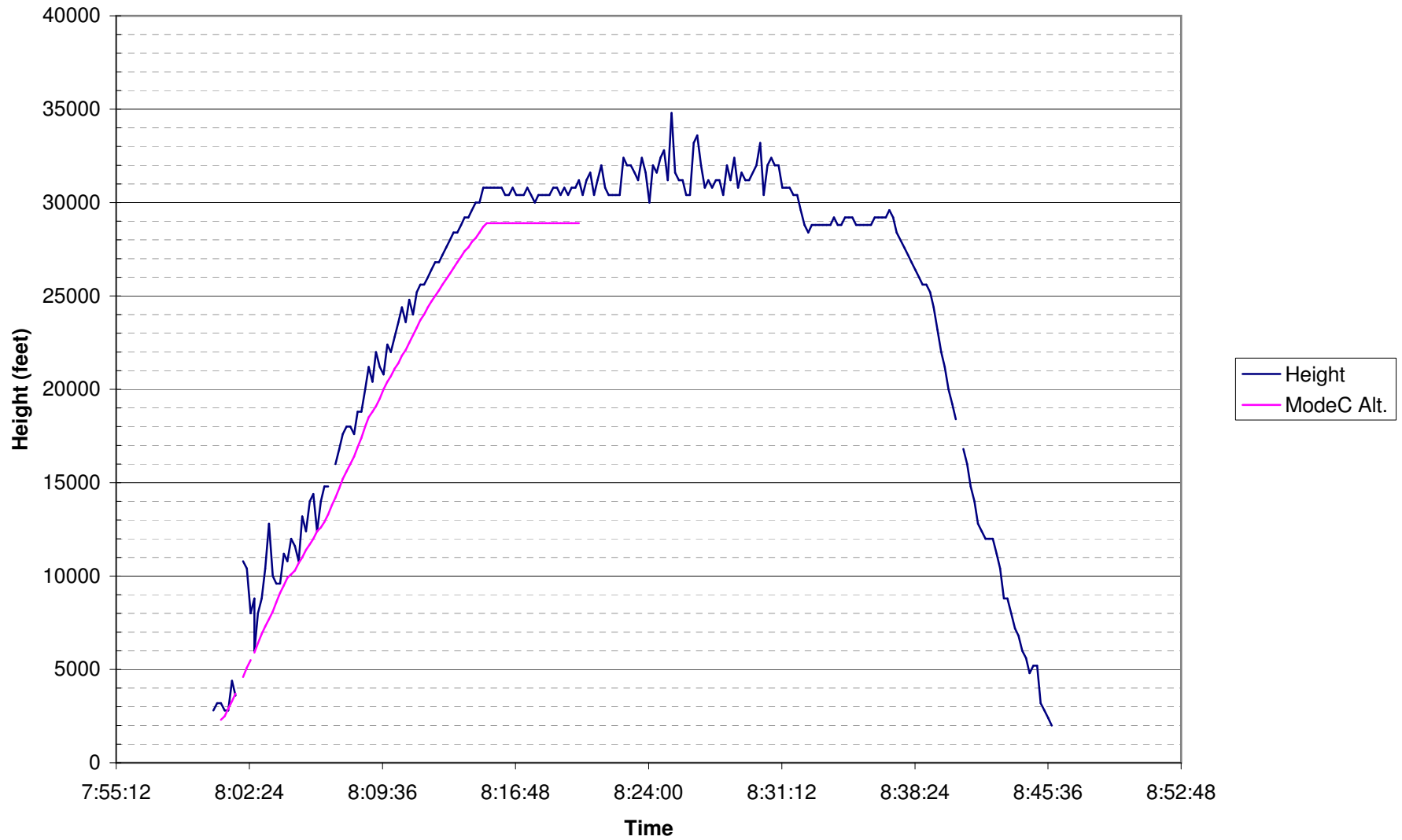
AA11 WTC1 North B767 Height & Mode C Altitude, Taken From USAF 84 RADES .XLS Data
